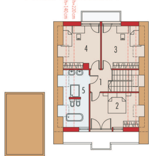
Plan MANSARDĂ
