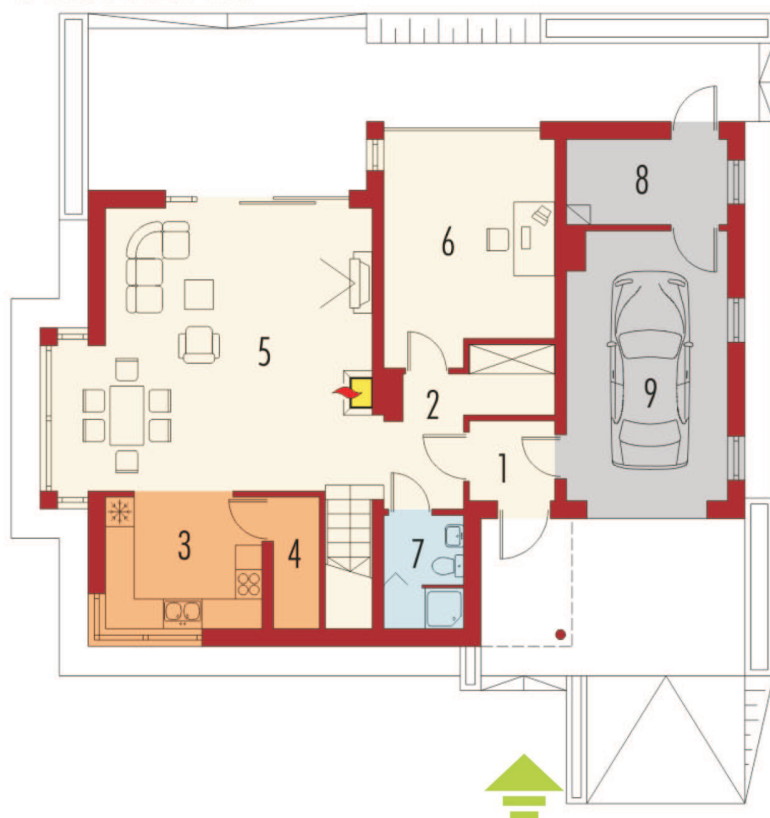
Plan PARTER
