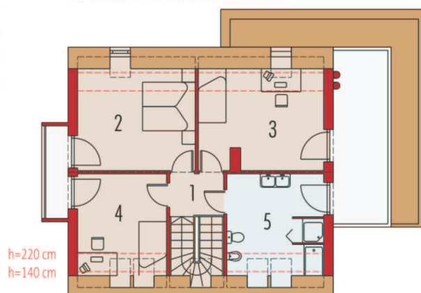
Plan MANSARDĂ
