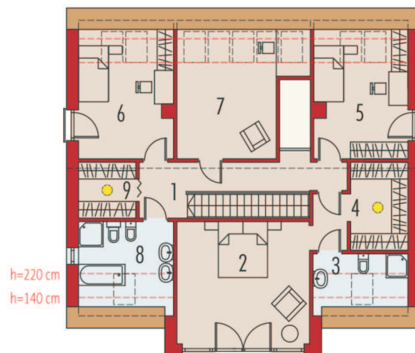
Plan MANSARDĂ
