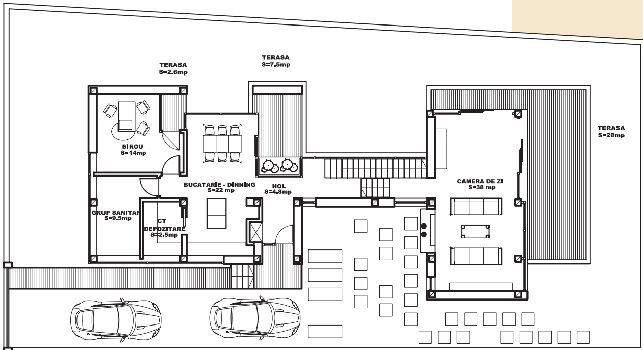
PLAN PARTER
